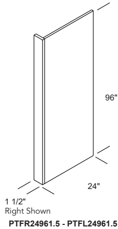
Laminate Tall Filler Panel (Slab)
