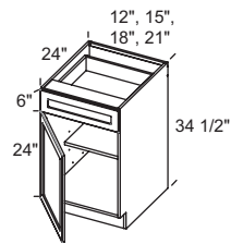
Left Shown B12(L/R) - B21FX(L/R)
