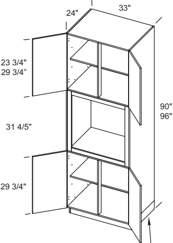
Toe Kick Sub Assembly OC3390 - OC3396
