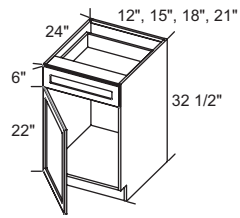
Left Shown B1232.5(L/R) - B2132.5FX(L/R)
