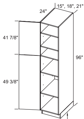
Left Shown Toe Kick Sub Assembly T1596(L/R) - T2196(L/R)
