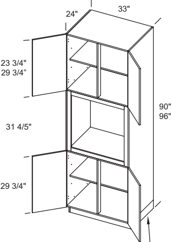
Toe Kick Sub Assembly OC3390 - OC3396
