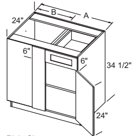
Right Shown BC36(L/R) - BC45FX(L/R)
