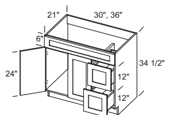
Right Shown VBSD30(L/R) - VBSD36FX(L/R)
