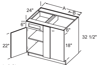
Left Shown BC3632.5(L/R) - BC4532.5FX(L/R)
