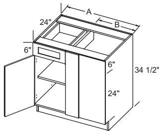
Left Shown BC36(L/R) - BC45FX(L/R)
