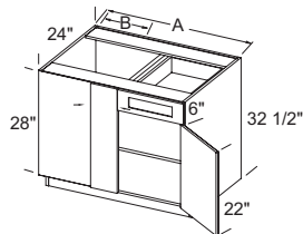
Right Shown BC3632.5(L/R) - BC4532.5FX(L/R)
