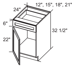
Left Shown B1232.5(L/R) - B2132.5FX(L/R)
