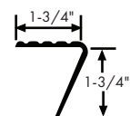
DTN-XX Top set stair nosing for residential use
