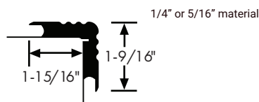
VCD-XX 1/4" or 5/16" material on step and riser
