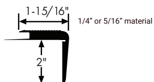
RCN-XX-A 1/4" or 5/16" material on step
